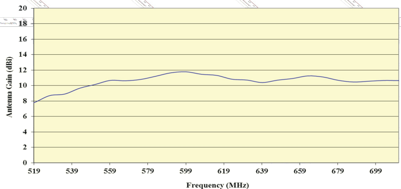
Antenna Gain (dBi) vs. Frequency (MHz)
