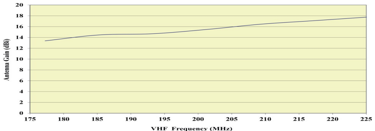
Antenna Gain (dBi) vs. Frequency (MHz)
