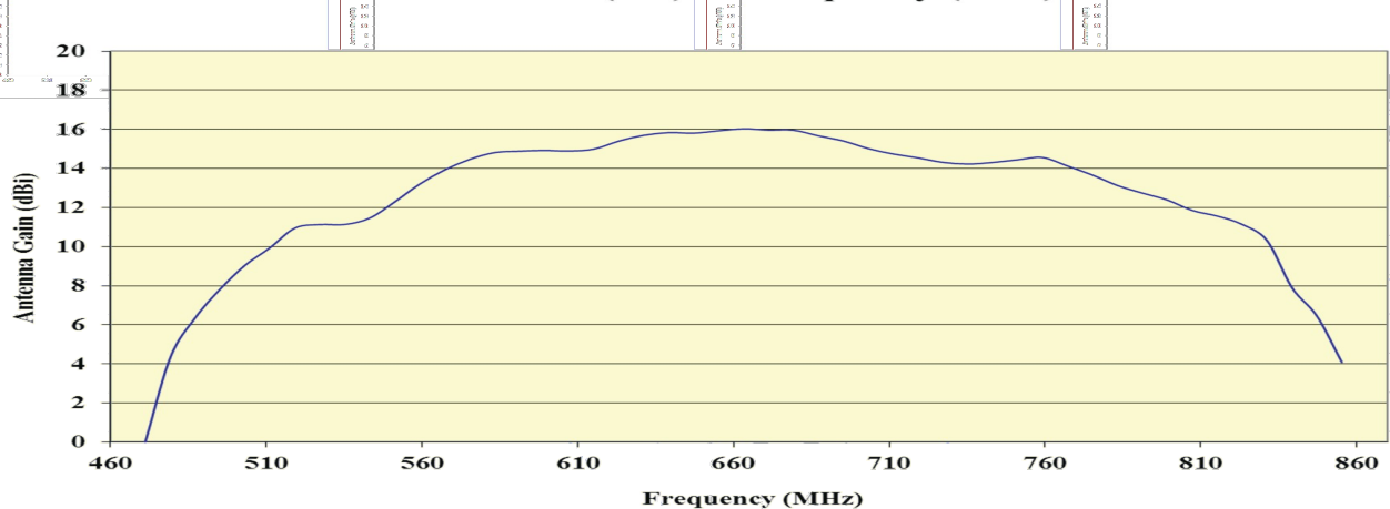
Antenna Gain (dBi) vs. Frequency (MHz)
