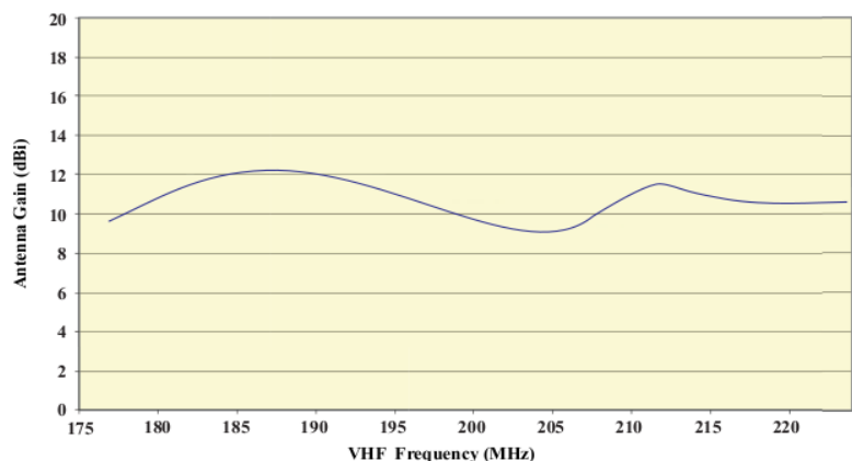
Antenna Gain (dBi) vs. Frequency (MHz)
